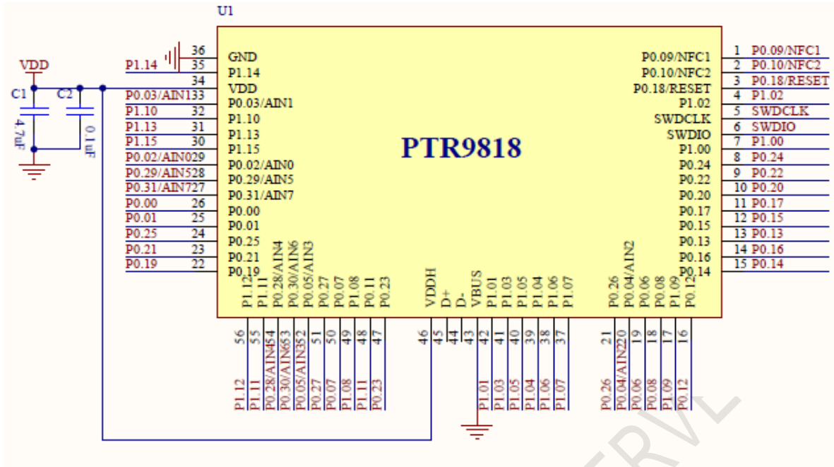
Configurations summary for reference circuit 4
