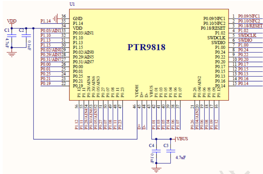
Configurations summary for reference circuit 3
