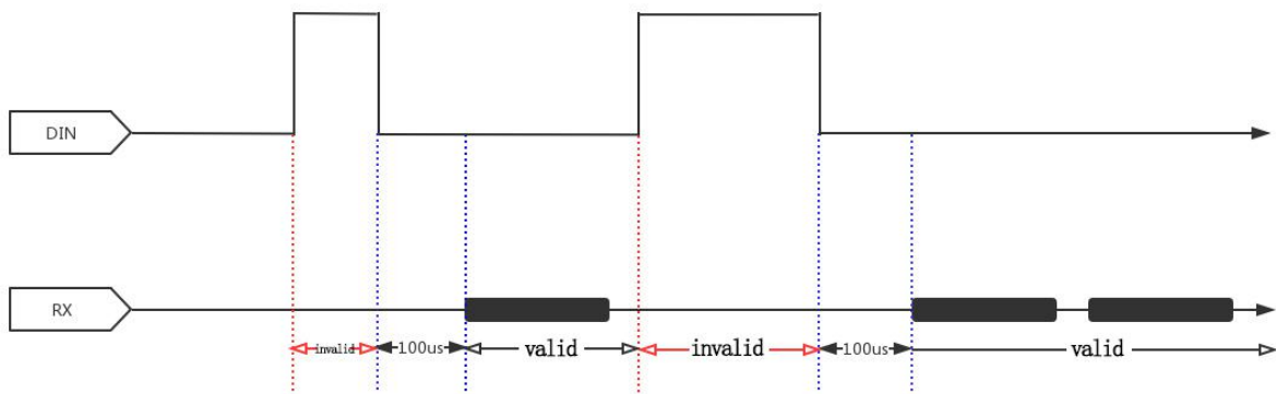
Figure 5 DIN timing sequence
