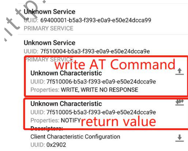
Figure 3 AT Command through air
